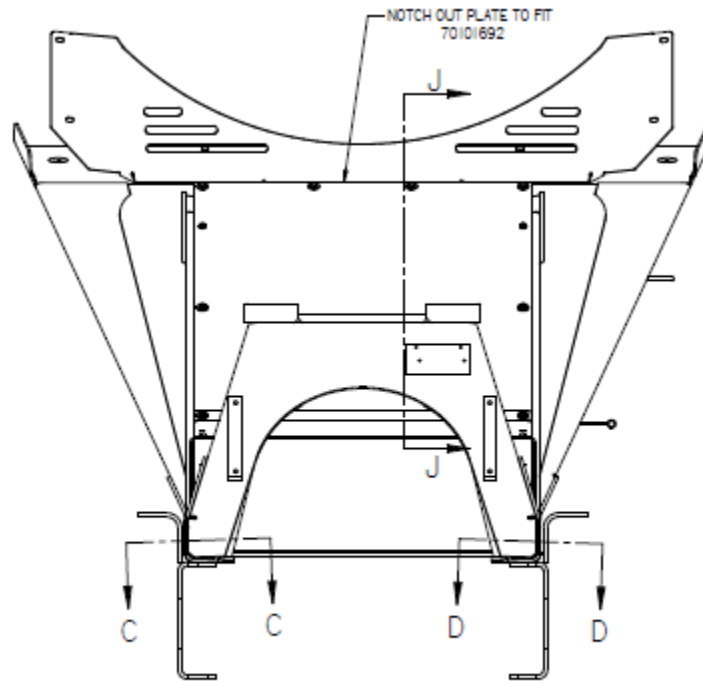
FRONT VIEW OF ASSEMBLY
